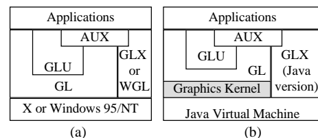
Figure 1. (a)The hierarchy of OpenGL modules. (b)The hierarchy of JavaGL modules.
